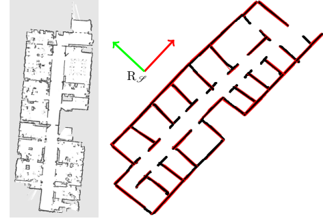
Fig. 4. Reference frame computed using the method described in Sec. III-B. On the left a SLAM image of an indoor building computed using the CARMEN framework [20]. On the right, the lab map sketched with our interface.
