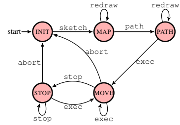
Fig. 3. A finite state machine depicting the tasks that a user can perform using the tablet interface.
