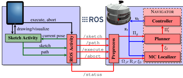
Fig. 2. System architecture showing the software components on the tablet and in the robot. As described in Sec III, \xi_t is the robot state. \Pi_g and \Pi'_t are respectively the global and local path, \mathbf{u}_t is the control and \mathbf{z}_t the measurements. (\Omega_{\mathcal{S}}, R_{\mathcal{S}}) is the sketched map.
