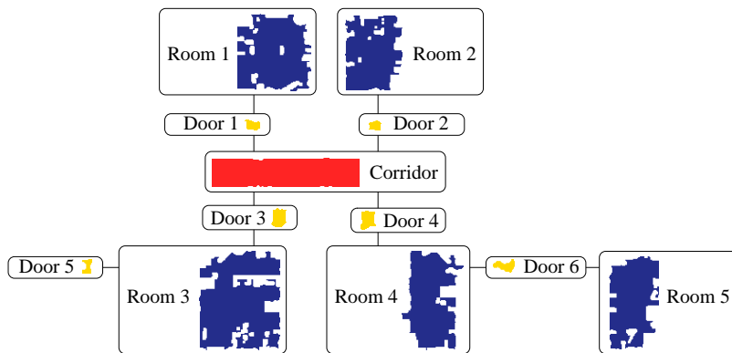
(c) Final topological map
