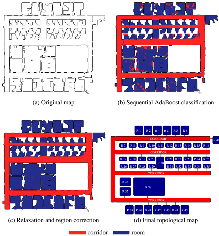
Fig. 13. This figure shows (a) the original map of the building, (b) the results of applying the sequential AdaBoost classifier with a classification rate of 92.4%, (c) the resulting classification after the relaxation and region correction, and (d) the final topological map with semantic information. The regions are omitted in each node. The rooms are numbered left to right and top to bottom with respect to the map in (a). For the sake of clarity, the corridor-node is drawn maintaining part of its region structure.
