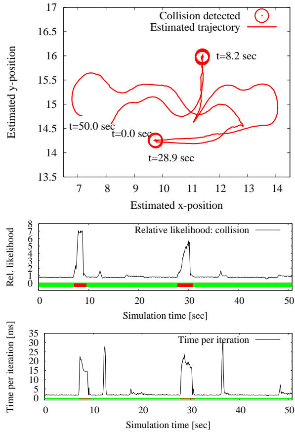
Fig. 5. A trajectory followed by a simulated robot (first row) with marks at positions where the evidence for a collision was high. The plot in the second row depicts the relative likelihood for collisions. The plot also shows the ground truth (the bar at the bottom). The last plot shows the time needed for each iteration (third row).
