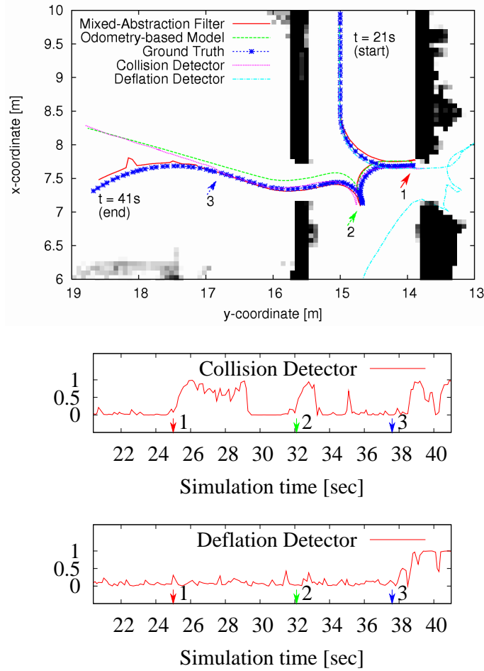
Fig. 4. Results of an experiment with two fault-events (top). The collision of the robot with a glass door is marked with “1”, the point where it stopped backing of and turned is marked with “2”, and at point “3” the left tire of the robot started losing air. The diagram in the middle plots the relative number of the particles in the fault mode of the collision detector. The lower diagram shows the corresponding number for the deflation detector.
