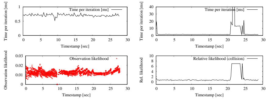
Fig. 6. In an experiment with a real robot, the observation likelihood of the standard system model (lower left) does not indicate the collision with a glass door at time t = 22 seconds. The mixed-abstraction particle filter (right) detects the fault without needing substantially more computational resources in the fault-free case (upper diagrams).
