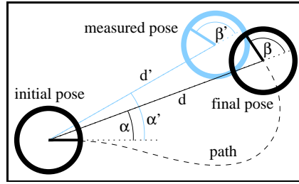
Fig. 3. Parameters of the standard odometry-based motion model.
